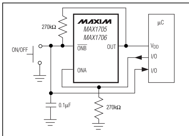
Figure 11. Momentary Pushbutton On/Off Switch
