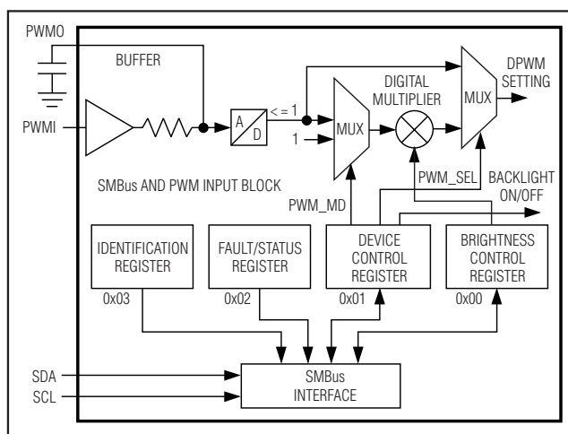
Figure 5. MAX17061 PWM and SMBus Interface Circuit
