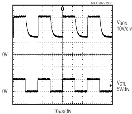
HIGH-VOLTAGE SWITCH CONTROL FUNCTION
