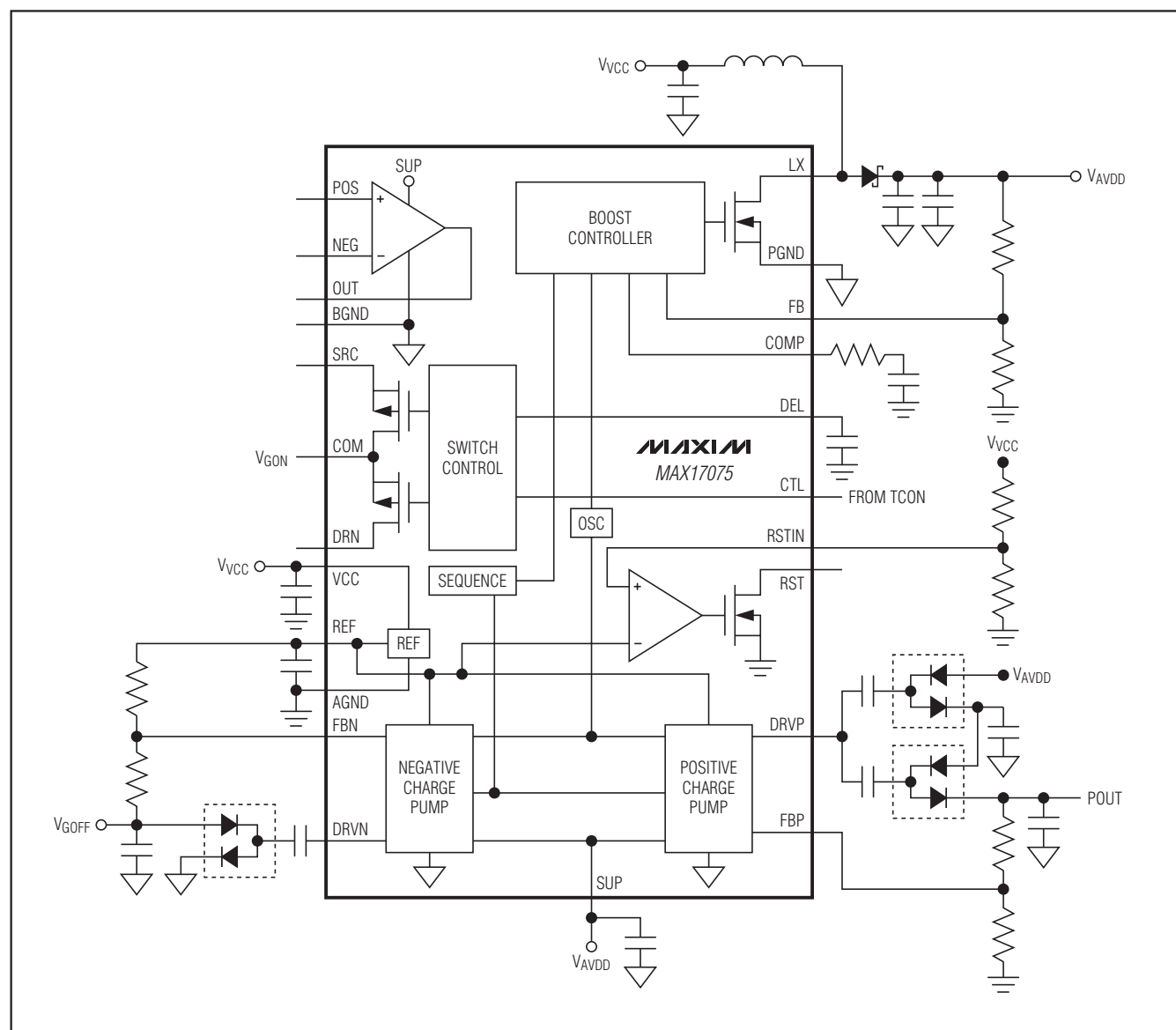
Figure 2. Functional Diagram
