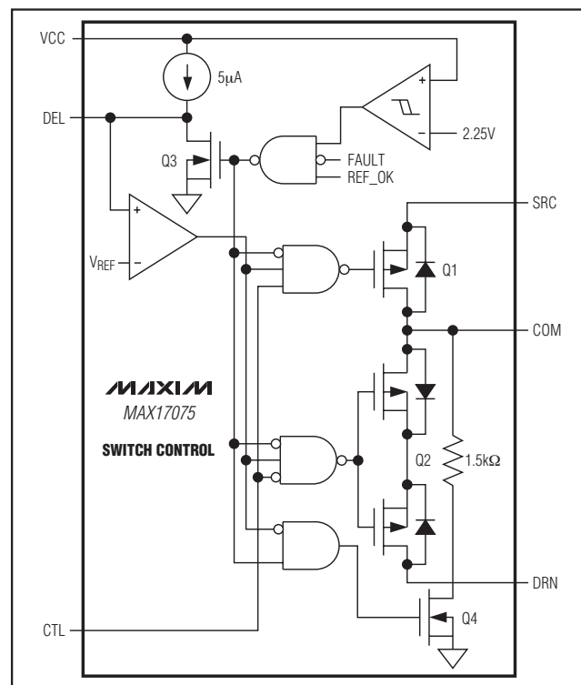
Figure 7. Switch Control
