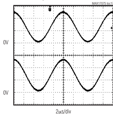
OPERATIONAL AMPLIFIER RAIL-TO-RAIL INPUT/OUTPUT WAVEFORMS
