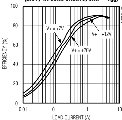
EFFICIENCY vs. LOAD CURRENT (2.5V, 4A COMPONENTS, \overline{SKIP} = V_{CC} )
