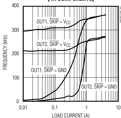
FREQUENCY vs. LOAD CURRENT (4A COMPONENTS)
