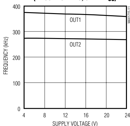
FREQUENCY vs. SUPPLY VOLTAGE (4A COMPONENTS, \overline{SKIP} = V_{CC} )
