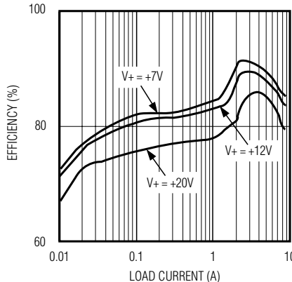
EFFICIENCY vs. LOAD CURRENT (1.3V, 8A COMPONENTS, \overline{SKIP} = GND )
