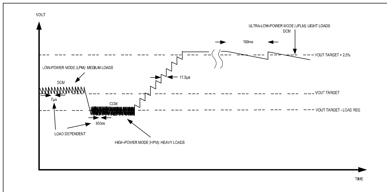
Figure 5. ULPM, LPM, and HPM Waveforms (Part 2).
