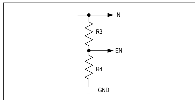
Figure 2. Setting the Minimum Operating Input Voltage
