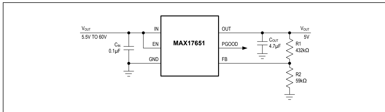
Figure 4. Application Circuit for 5V output
