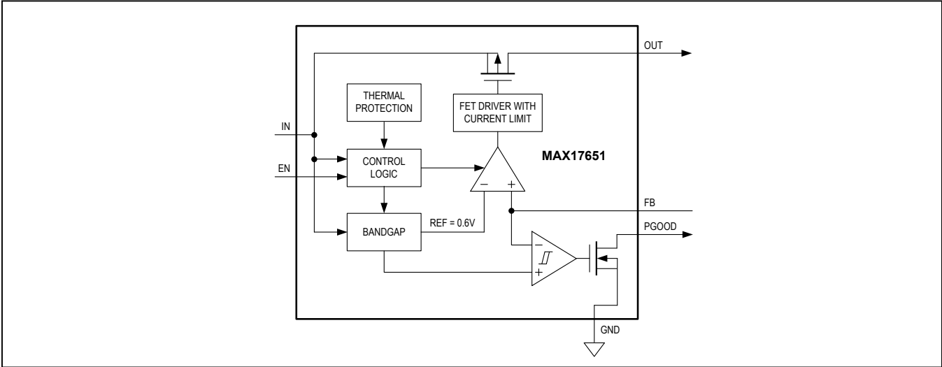
Figure 1. Block Diagram
