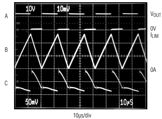
MEDIUM-LOAD SWITCHING WAVEFORMS
