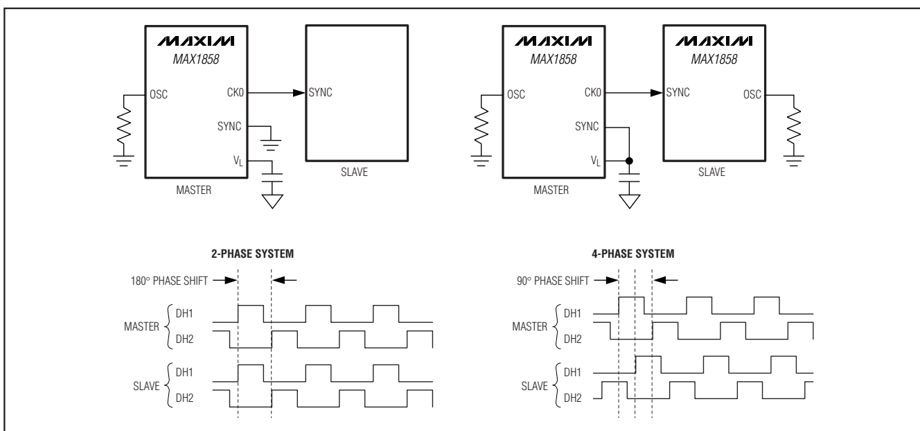
Figure 5. Synchronized Controllers
