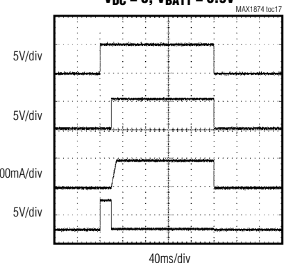
USB CONNECT WAVEFORMS V_DC = 0, V_BATT = 3.9V
