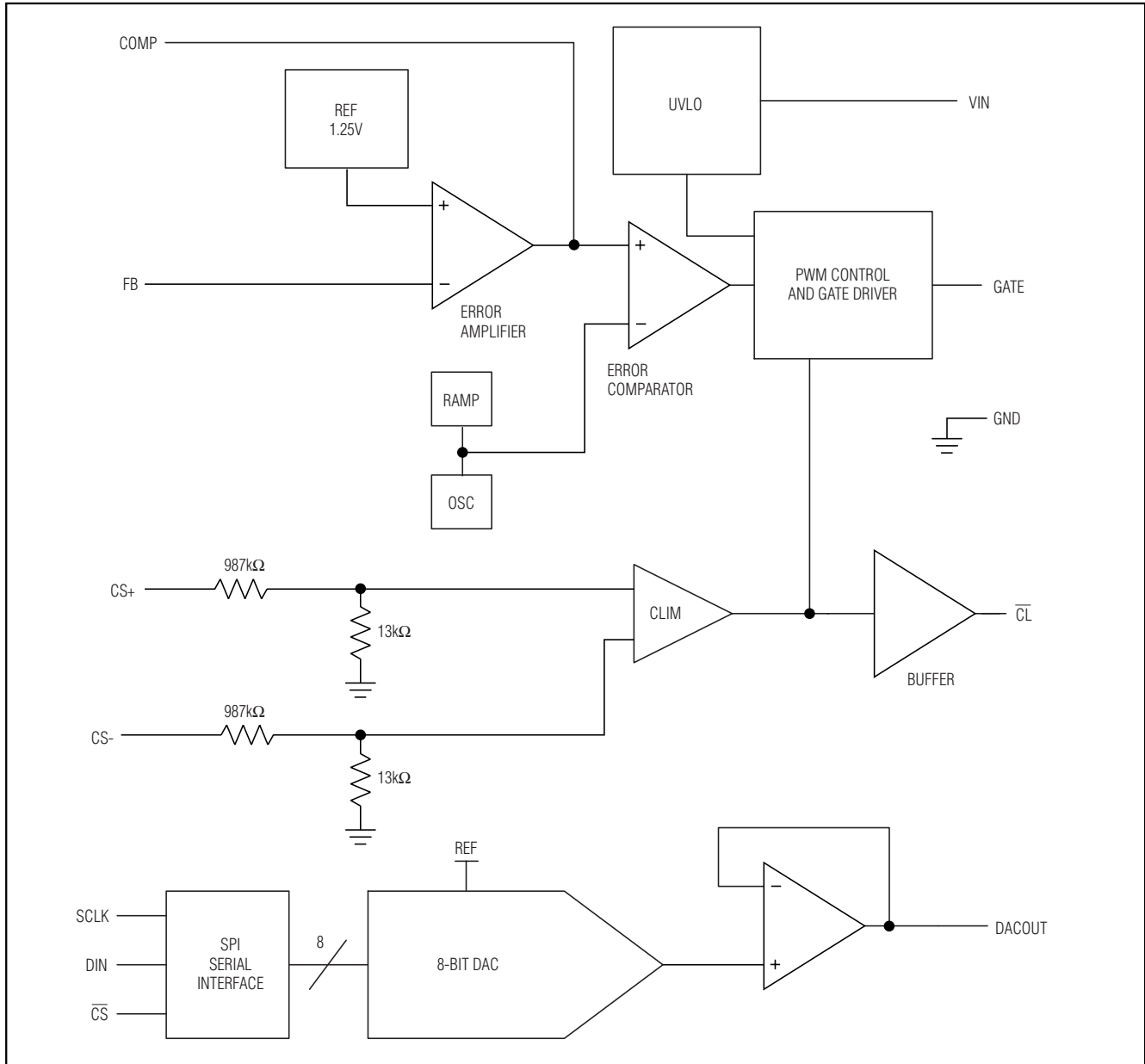
Figure 1. Functional Diagram
