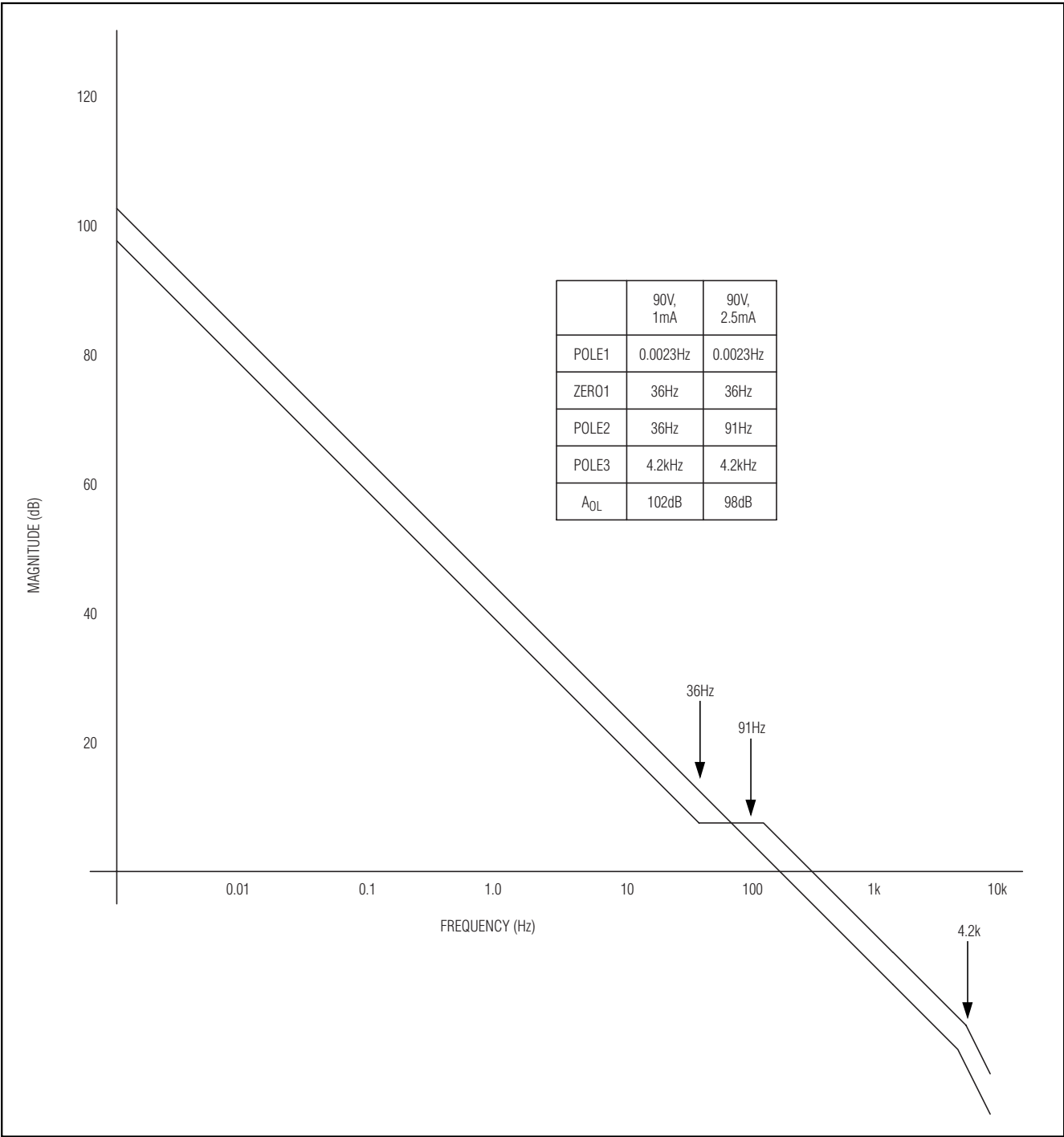
Figure 6. Loop Response
