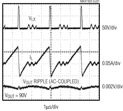
SWITCHING WAVEFORMS
