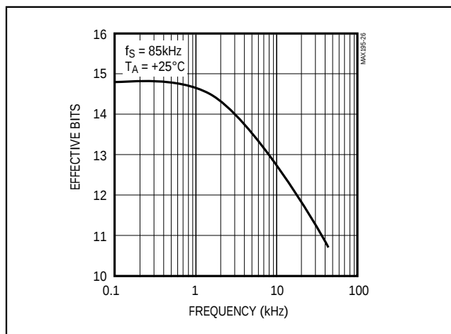
Figure 26. Effective Bits vs. Input Frequency
