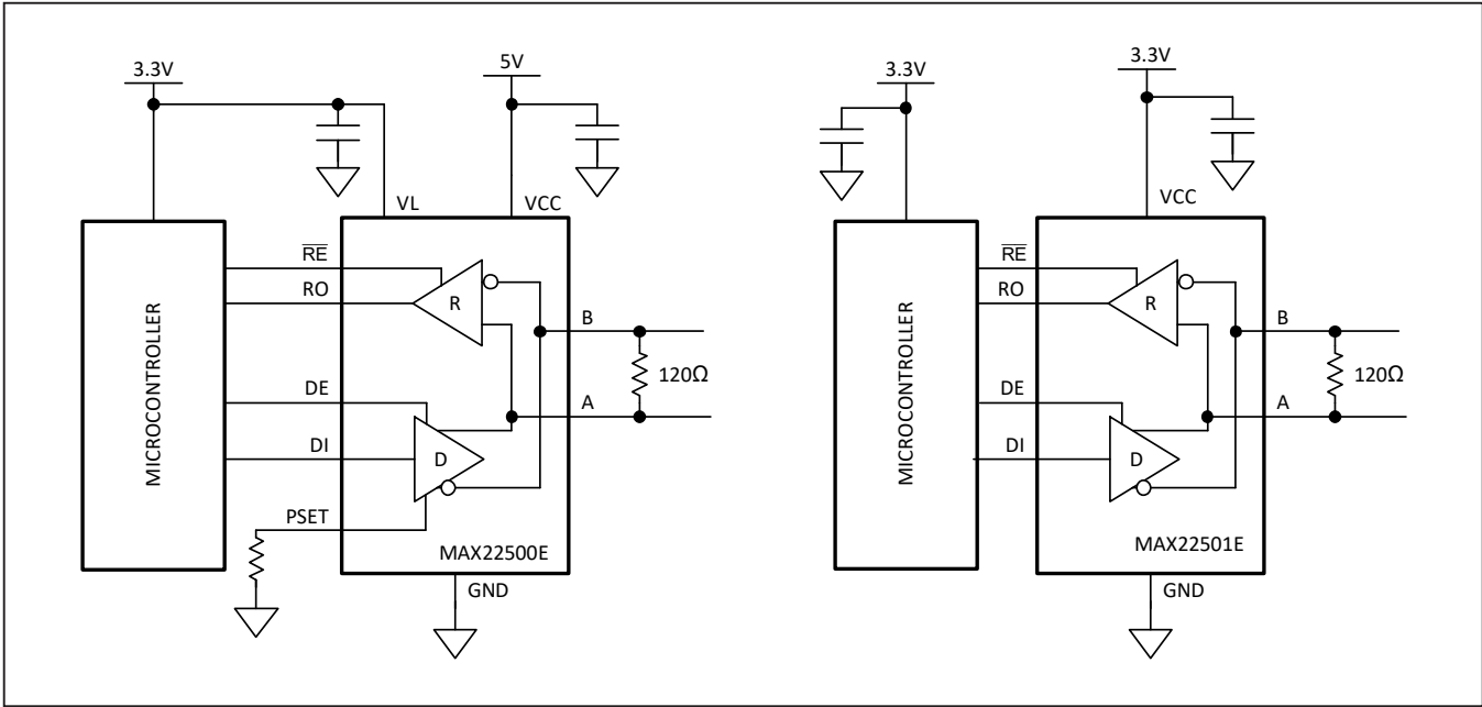
Half-Duplex Application Circuit
