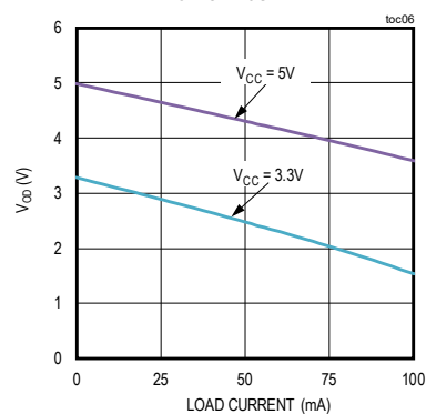
DIFFERENTIAL DRIVER OUTPUT VOLTAGE vs. LOAD CURRENT
