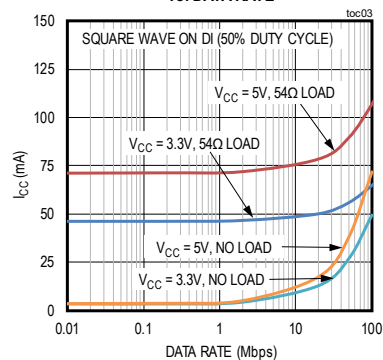
MAX22501E SUPPLY CURRENT vs. DATA RATE
