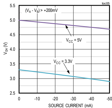
RO OUTPUT VOLTAGE HIGH vs. LOAD CURRENT
