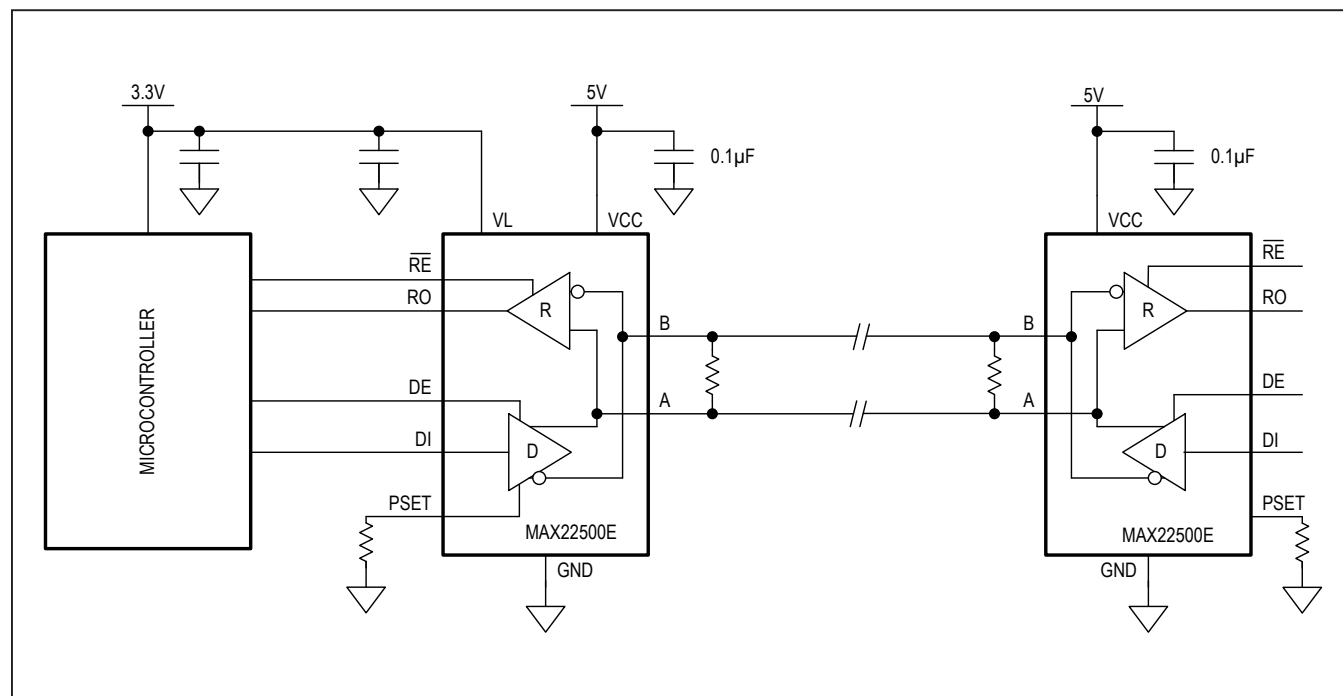
Figure 16: Point-to-Point Half-Duplex Communication for High Speeds
