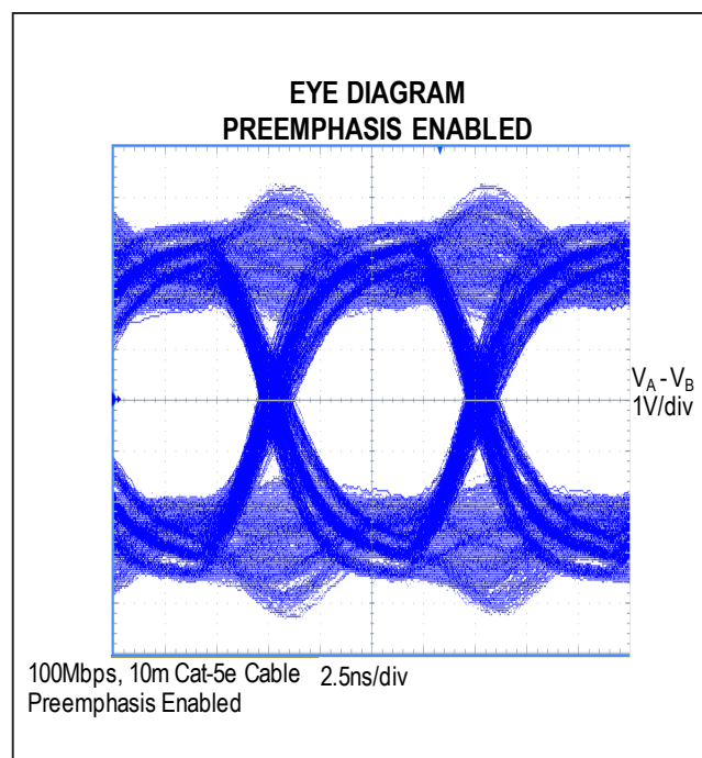
Figure 11: Eye Diagram, 100Mbps Over 10m Cat-5e Cable, Preemphasis Enabled
