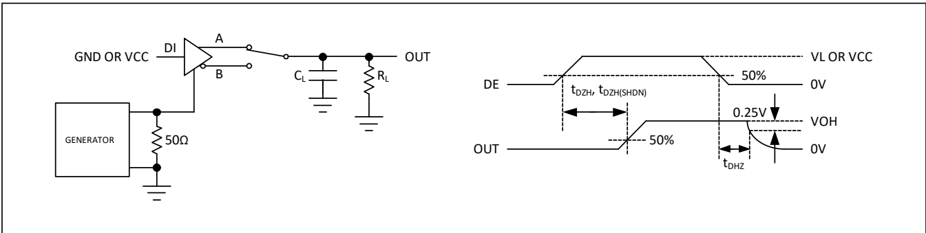
Figure 5: Driver Enable and Disable Times ( t_{DZH} , t_{DHZ} )
