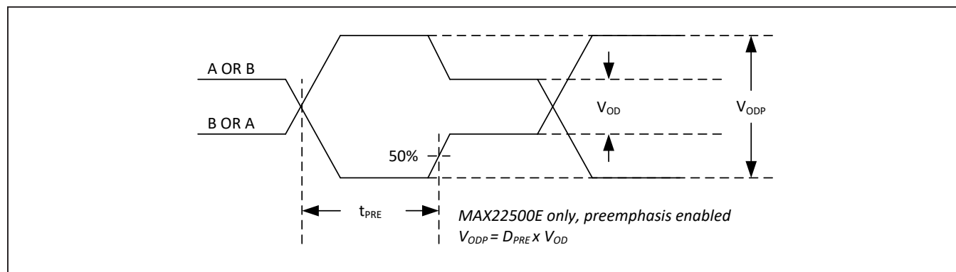
Figure 2: Driver Preemphasis Timing
