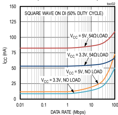
MAX22500E SUPPLY CURRENT vs. DATA RATE (PREEMPHASIS DISABLED)
