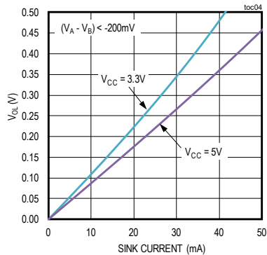
RO OUTPUT VOLTAGE LOW vs. LOAD CURRENT
