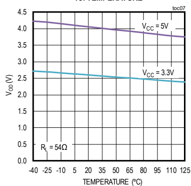
DIFFERENTIAL DRIVER OUTPUT VOLTAGE vs. TEMPERATURE
