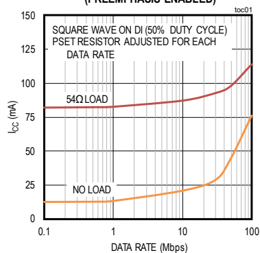
MAX22500E SUPPLY CURRENT vs. DATA RATE (PREEMPHASIS ENABLED)
