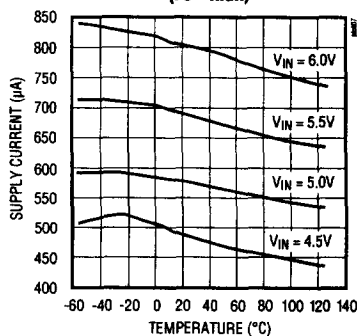
SUPPLY CURRENT vs. TEMPERATURE (FS = HIGH)
