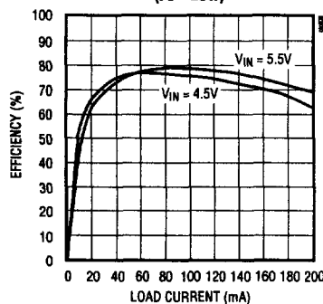
EFFICIENCY vs. LOAD CURRENT (FS = LOW)
