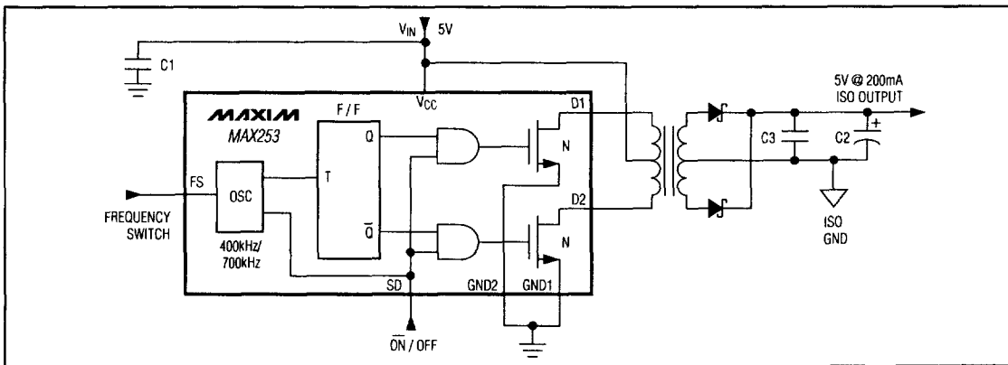
Figure 2. Block Diagram
