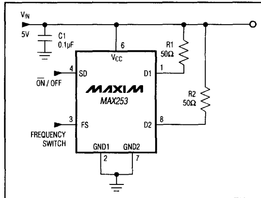
Figure 1. Test Circuit
