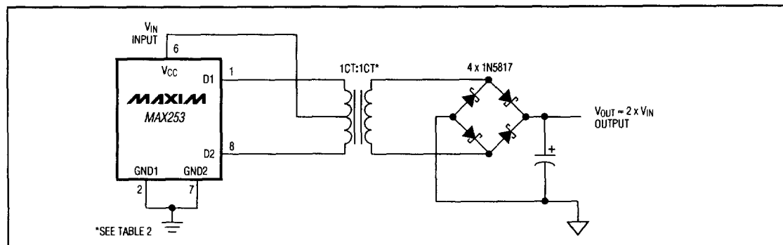
Figure 9c. Full-Wave Rectifier—Unipolar
