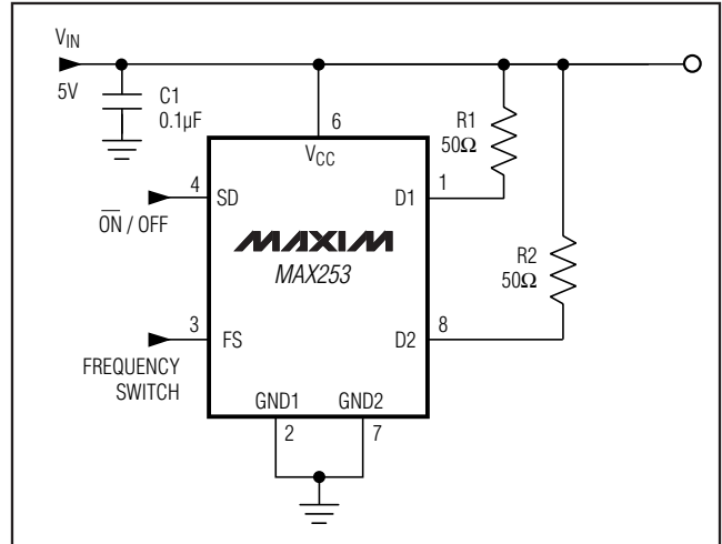
Figure 1. Test Circuit
