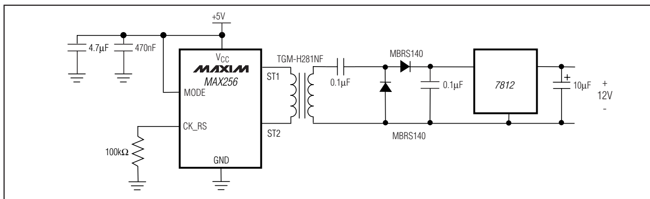
Figure 4. +5V to Isolated Regulated +12V
