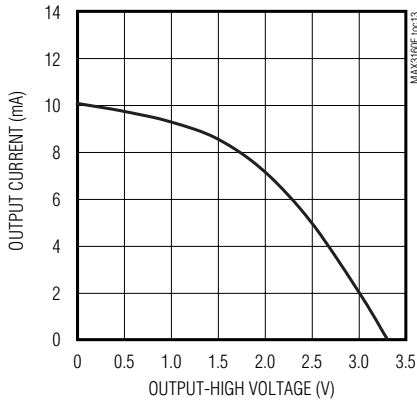
RECEIVER OUTPUT CURRENT vs. RECEIVER-OUTPUT HIGH VOLTAGE
