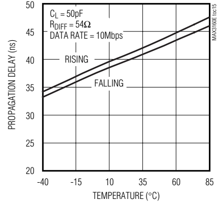
RS-485/RS-422 DRIVER PROPAGATION DELAY vs. TEMPERATURE (FAST = V_{CC} )
