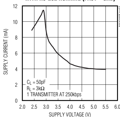
SUPPLY CURRENT vs. SUPPLY VOLTAGE WITH RS-232 RUNNING (FAST = GND)
