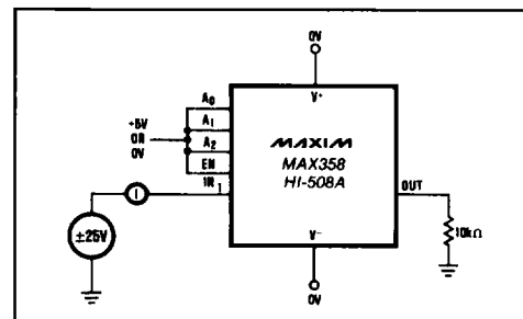
Figure 6. Input Leakage Current (with Power Supplies OFF)
