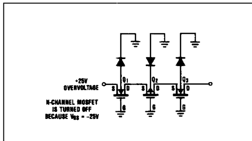
Figure 9. +25\text{V} Overvoltage with Multiplexer Power OFF
