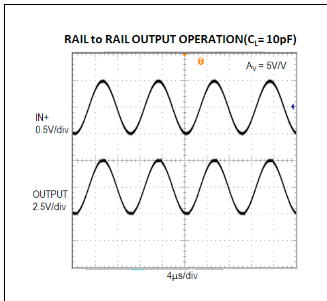
Figure 3. Rail-to-Rail Output Operation with 10kΩ
