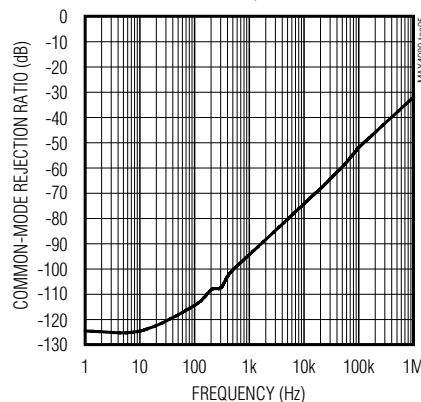
MAX4081F/T/S COMMON-MODE REJECTION RATIO vs. FREQUENCY
