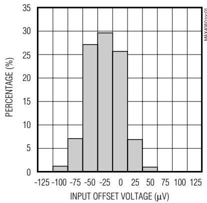
INPUT OFFSET VOLTAGE HISTOGRAM
