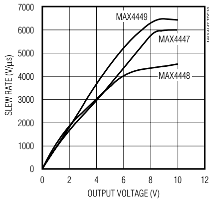
SLEW RATE vs. OUTPUT VOLTAGE
