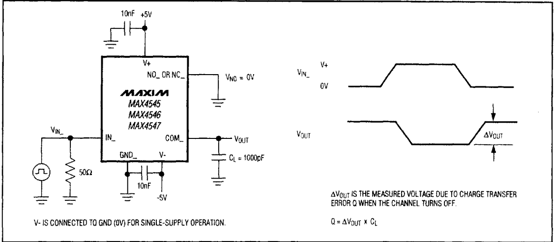
Figure 6. Charge Injection
