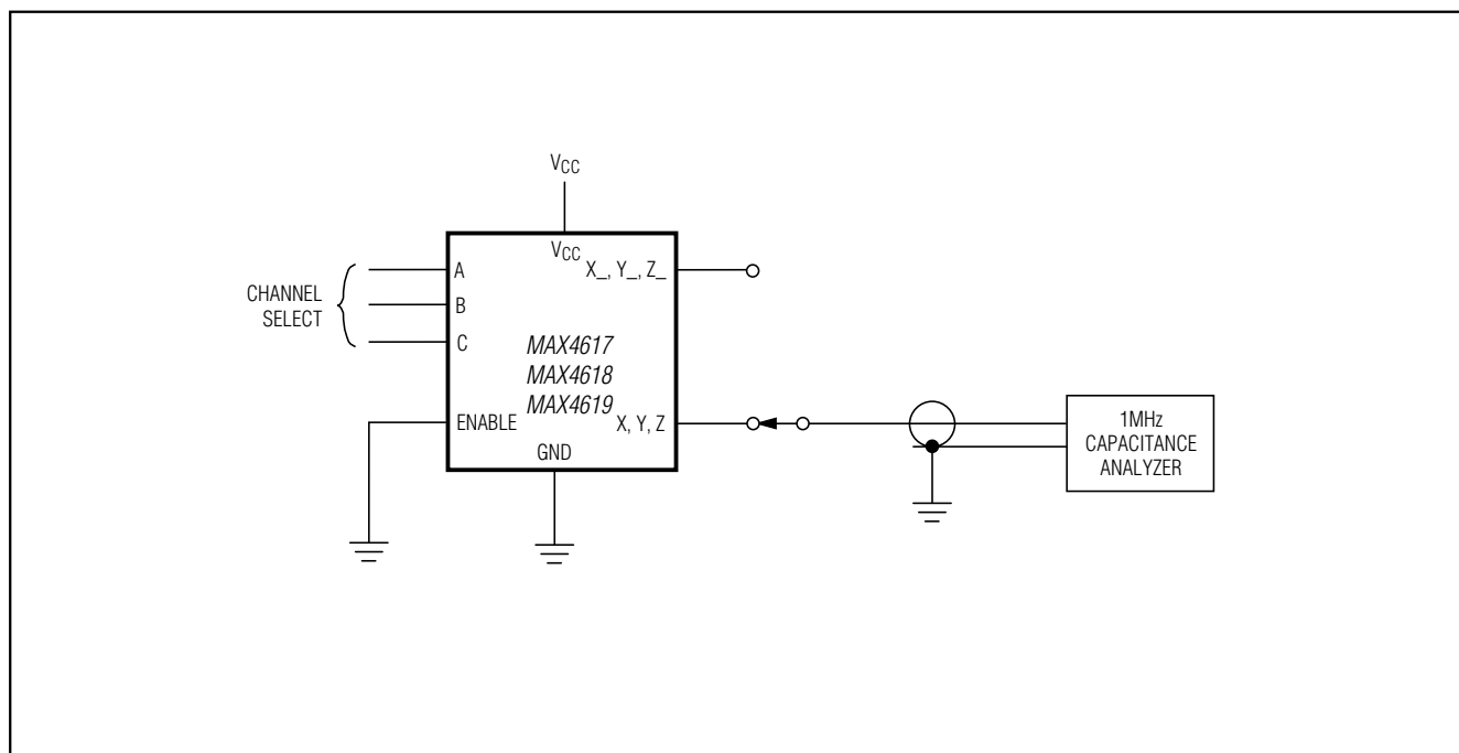
Figure 7. Capacitance
