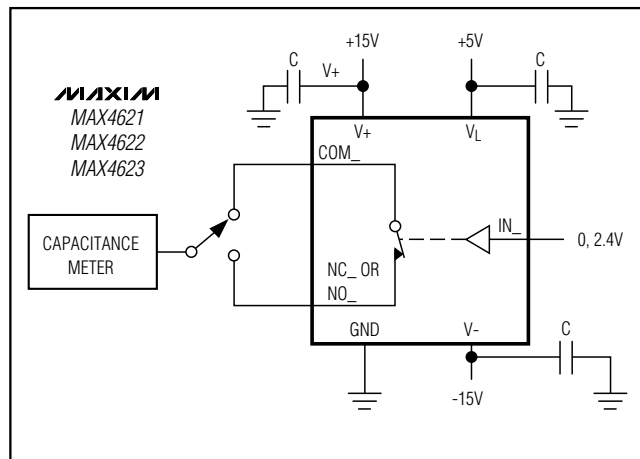
Figure 8. Channel-Off Capacitance
