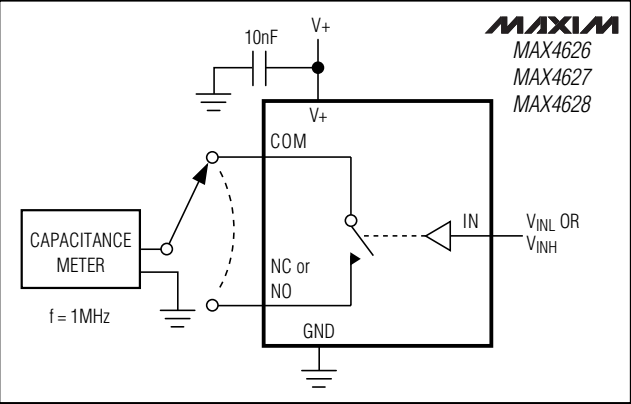
Figure 5. Channel Off/On-Capacitance
