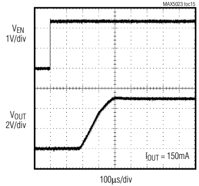
ENABLE STARTUP RESPONSE ( V_{IN} = +65V )
