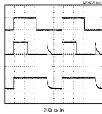
ENABLE AND HOLD TIMING
