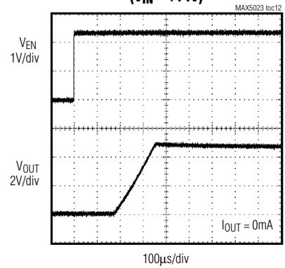
ENABLE STARTUP RESPONSE ( V_{IN} = +14V )
