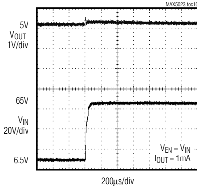
INPUT VOLTAGE STEP RESPONSE
