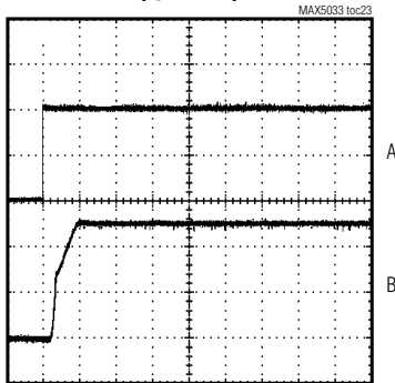
MAX5033BASA STARTUP WAVEFORM ( I_0 = 0.5A )
