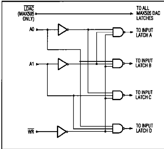
Figure 2. MAX505/MAX506 Input Control Logic
