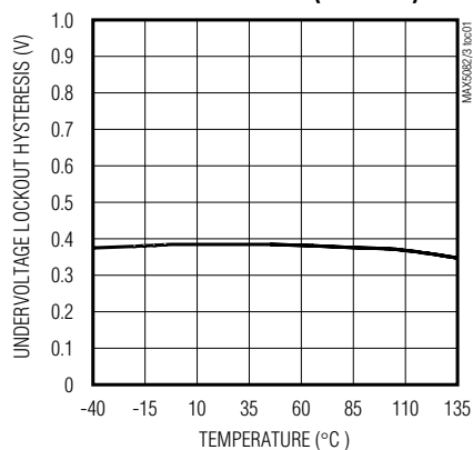
UNDervoltage LOCKOUT HYSTERESIS vs. TEMPERATURE (MAX5082)
