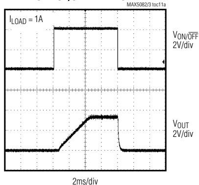
TURN-ON/OFF WAVEFORM
