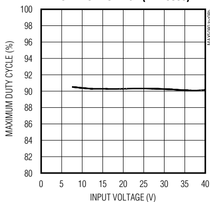
MAXIMUM DUTY CYCLE vs. INPUT VOLTAGE (MAX5083)
