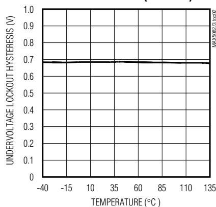
UNDervoltage LOCKOUT HYSTERESIS vs. TEMPERATURE (MAX5083)
