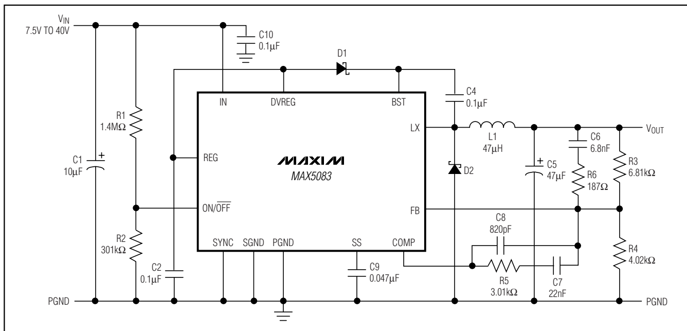
Figure 6. MAX5083 Typical Application Circuit
