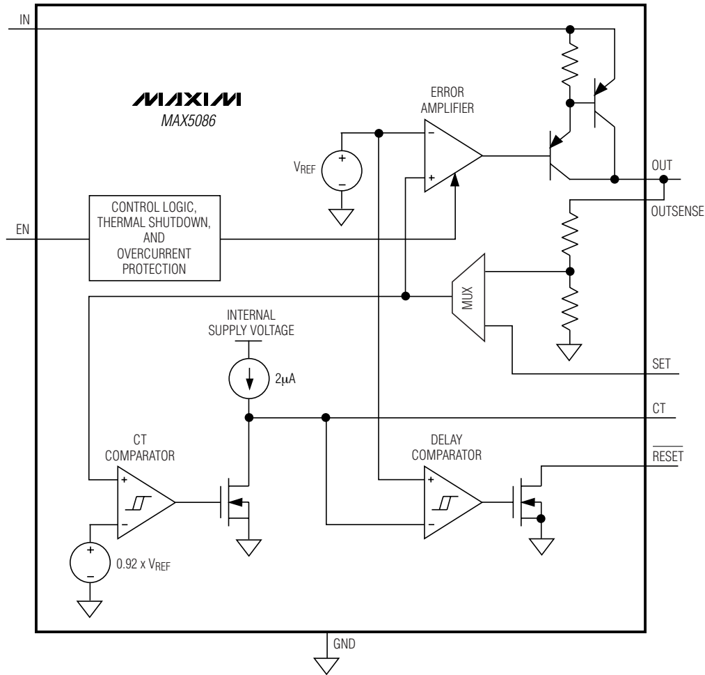
Figure 1. Functional Diagram
