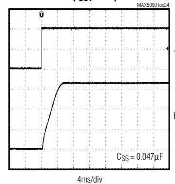
STARTUP WAVEFORM ( I_{OUT} = 2A )
