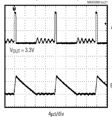
LX WAVEFORMS (MAX5090AATE)
