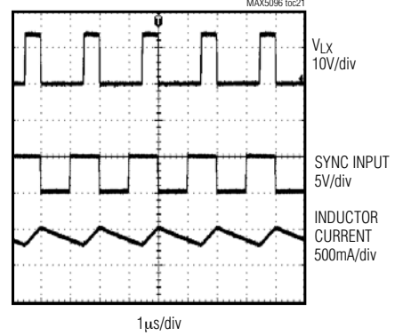
LX VOLTAGE, SYNC INPUT, AND INDUCTOR CURRENT
