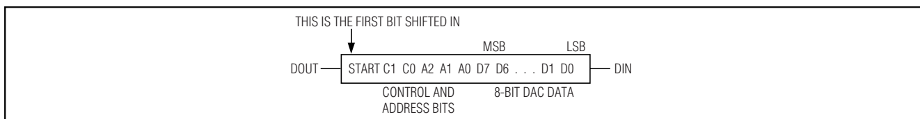
Figure 4. Serial Input Format
