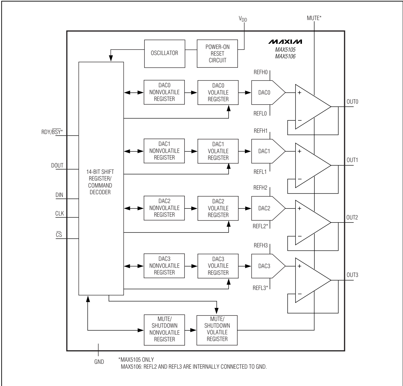
Functional Diagram
