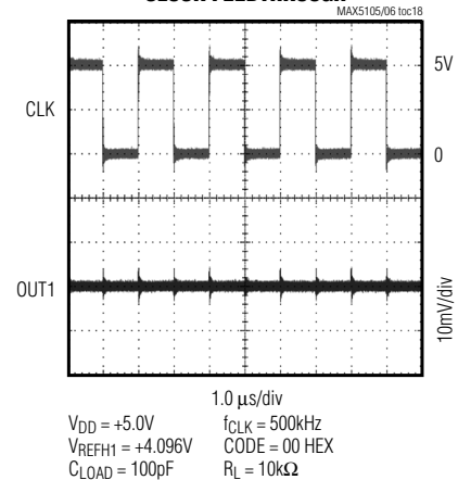
CLOCK FEEDTHROUGH
