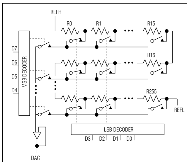
Figure 1. DAC Simplified Circuit Diagram
