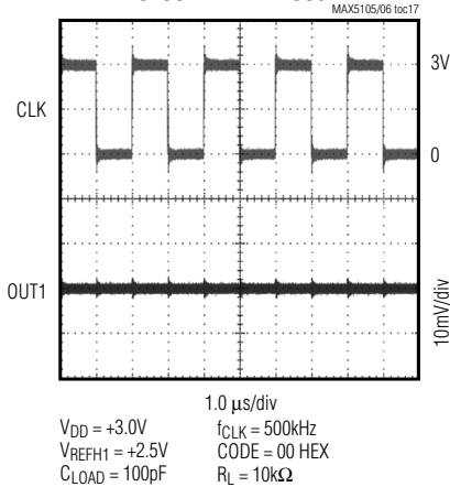
CLOCK FEEDTHROUGH
