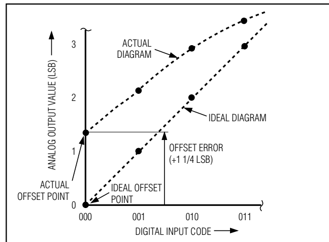
Figure 8c. Offset Error
