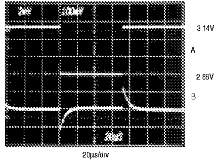
LINE-TRANSIENT RESPONSE (OUTC)
