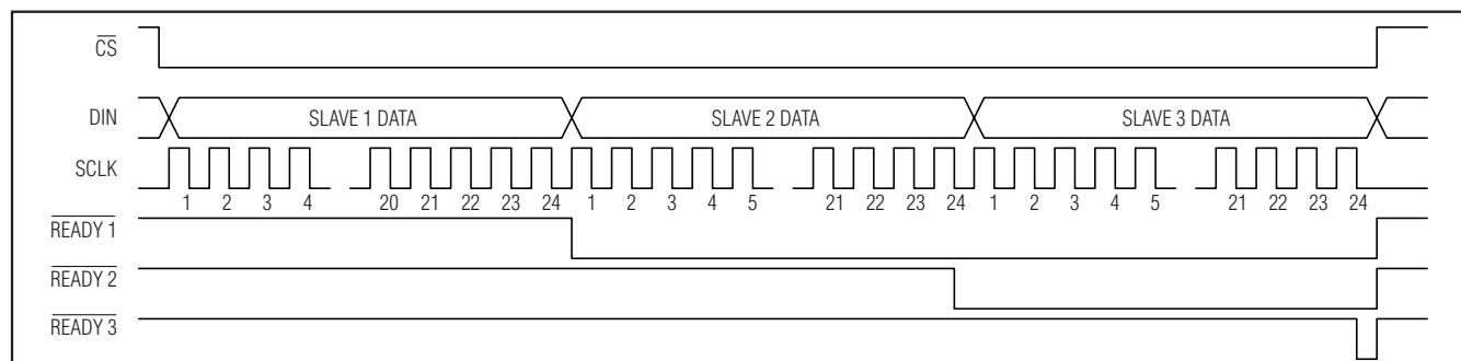
Figure 4. \overline{\text{READY}} Timing
