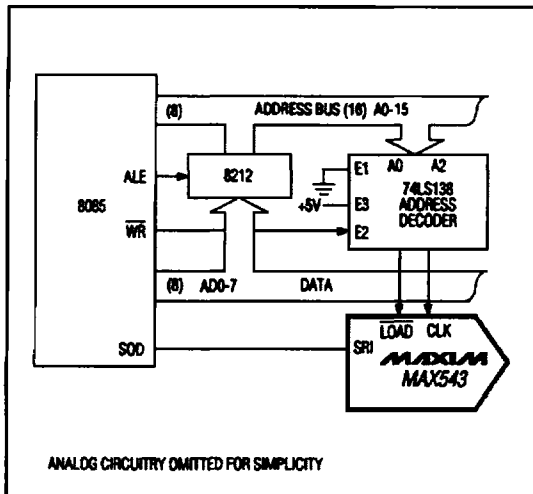
Figure 7. MAX543 8085 Interface
