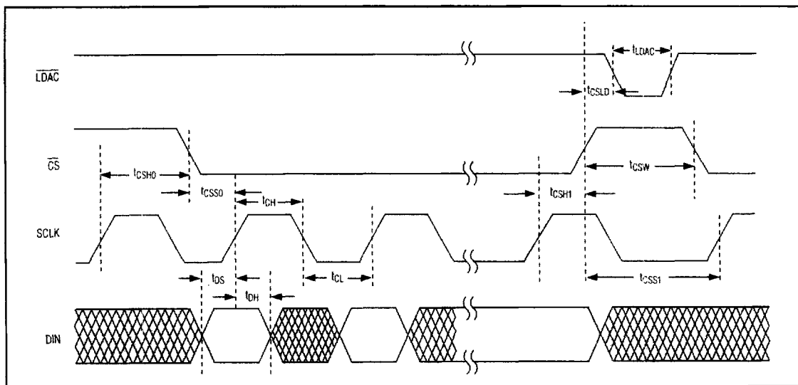
Figure 3. Detailed Serial-Interface Timing Diagram
