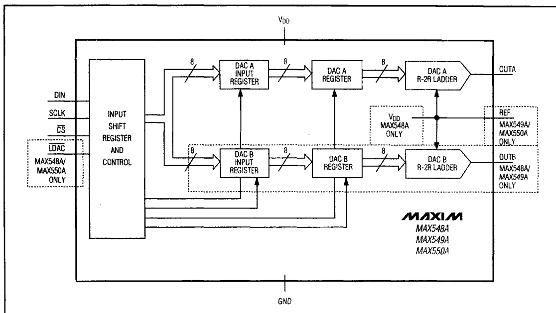
Functional Diagram
