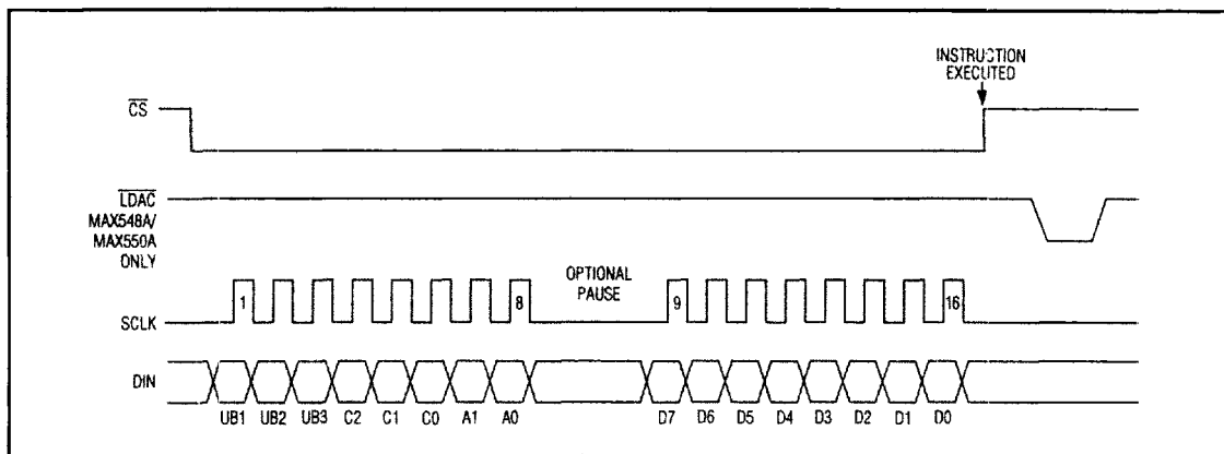
Figure 2. Serial-Interface Timing Diagram
