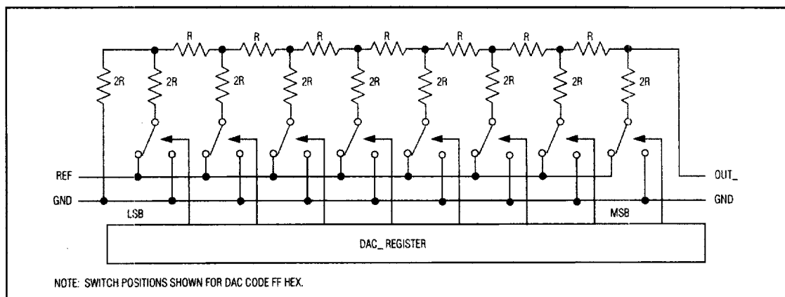
Figure 1. DAC Simplified Circuit Diagram
