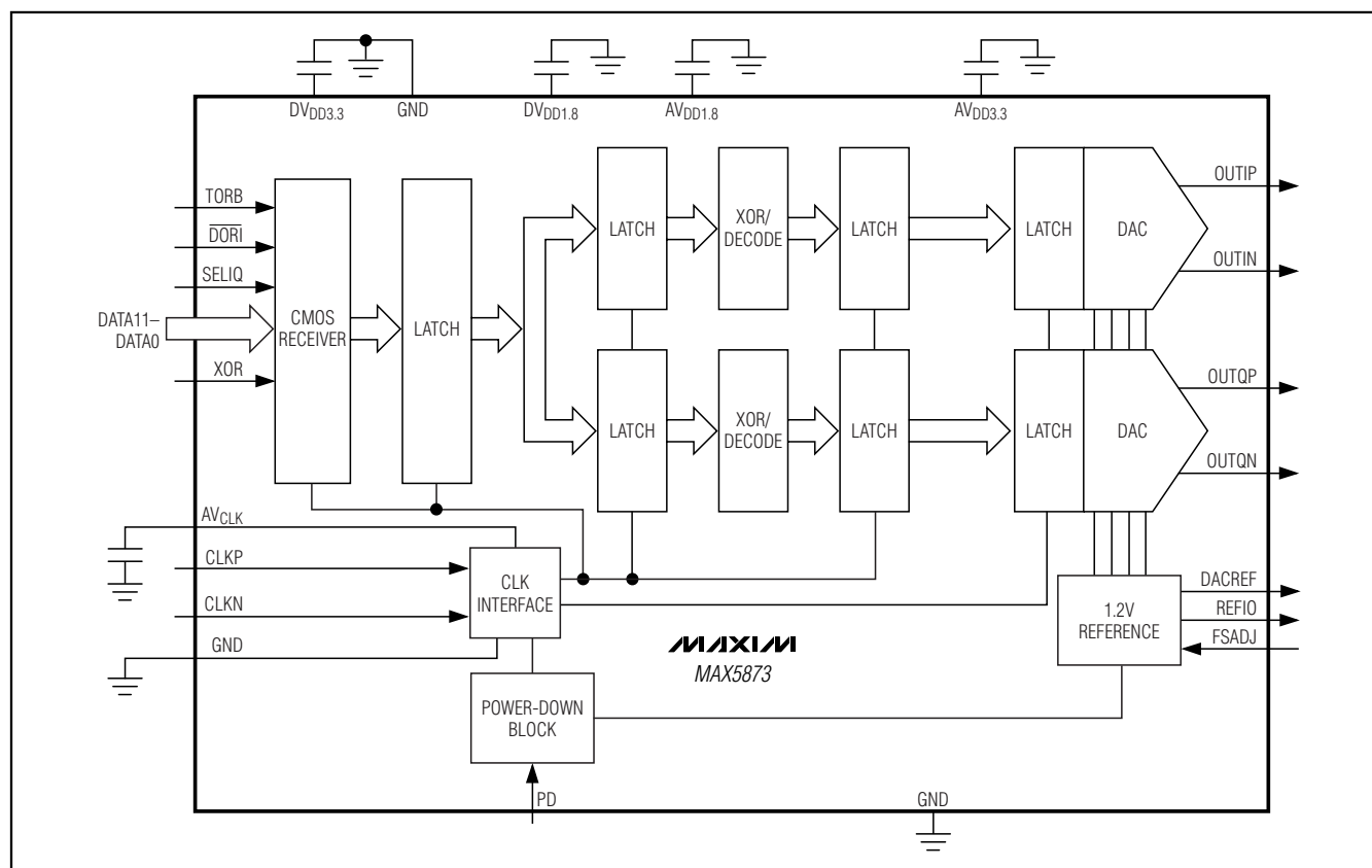
Figure 1. MAX5873 High-Performance, 12-Bit, Dual Current-Steering DAC
