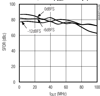
SINGLE-TONE SFDR vs. OUTPUT FREQUENCY ( f_{CLK} = 200Msps )
