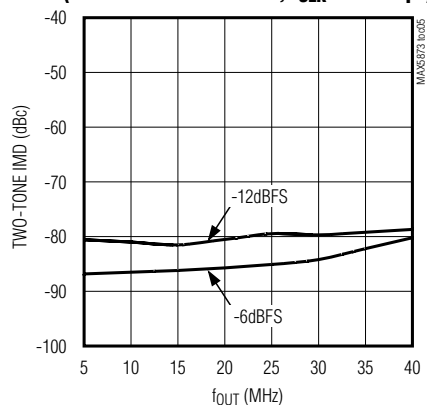
TWO-TONE IMD vs. OUTPUT FREQUENCY (1MHz CARRIER SPACING, f_{CLK} = 100Msps )
