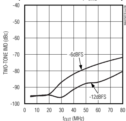
TWO-TONE IMD vs. OUTPUT FREQUENCY (1MHz CARRIER SPACING, f_{DAC} = 200Mps )
