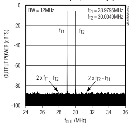
TWO-TONE INTERMODULATION DISTORTION ( f_{DAC} = 100Mps )
