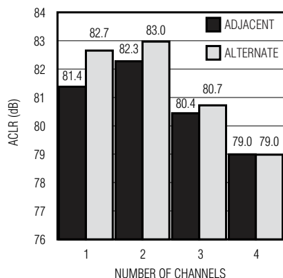
WCDMA BASEBAND ACLR
