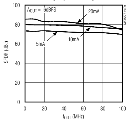
SFDR vs. FULL-SCALE OUTPUT CURRENT ( f_{DAC} = 200MHz )
