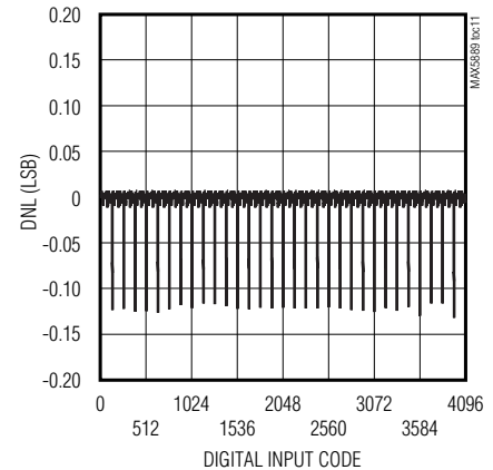
DIFFERENTIAL NONLINEARITY
