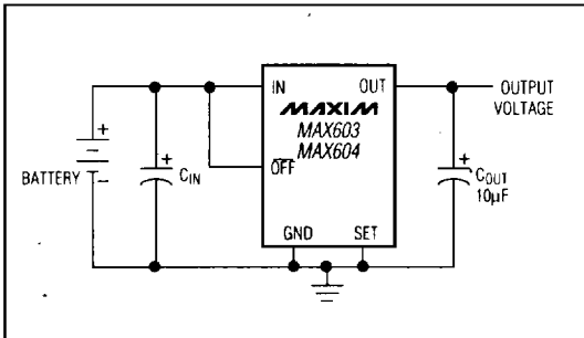
Figure 6. 3.3V or 5V Linear-Regulator Application
