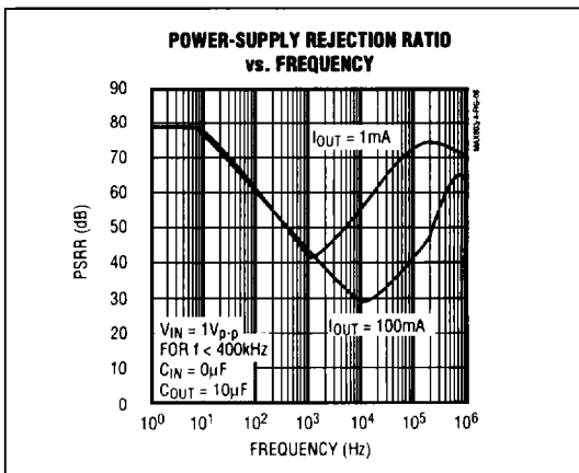
Figure 7. Power-Supply Rejection Ratio vs. Ripple Frequency
