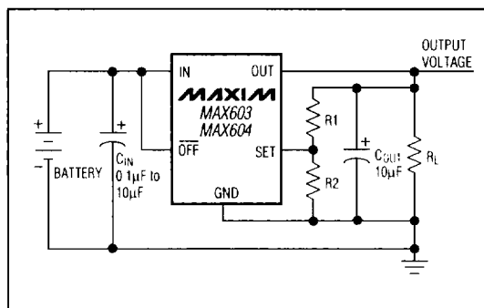
Figure 3. Adjustable Output Using External Feedback Resistors
