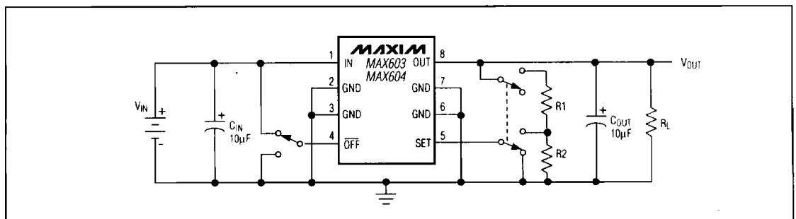
Figure 1. Test Circuit
