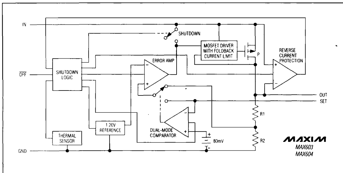
Figure 2. Functional Diagram
