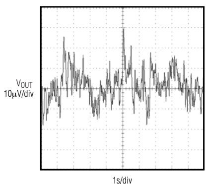
MAX6165 NOISE
