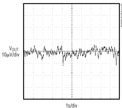
MAX6161 0.1Hz TO 10Hz OUTPUT NOISE
