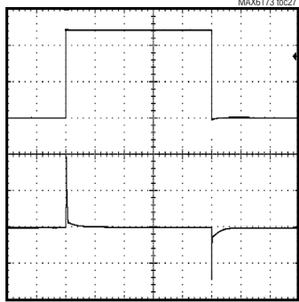
LOAD TRANSIENT ( V_{OUT} = 2.5V , C_{OUT} = 0 , 0 TO 20mA)
