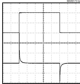
LOAD TRANSIENT ( V_{OUT} = 10V , C_{OUT} = 0 , 0 TO -2mA)
