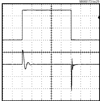
LOAD TRANSIENT ( V_{OUT} = 2.5V , C_{OUT} = 1\mu F , 0 TO +20mA)
