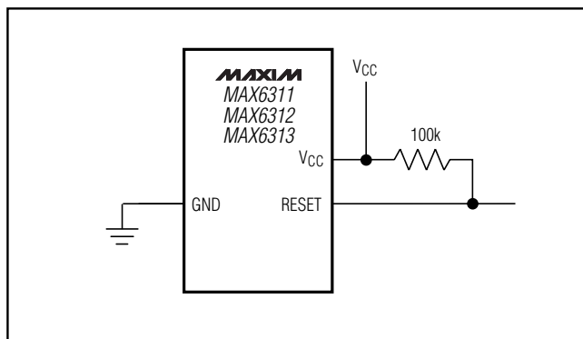
Figure 5. Ensuring \overline{\text{RESET}} Valid to V_{CC} = 0\text{V}
