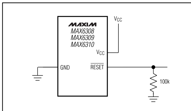
Figure 4. Ensuring \overline{\text{RESET}} Valid to V_{CC} = 0\text{V}
