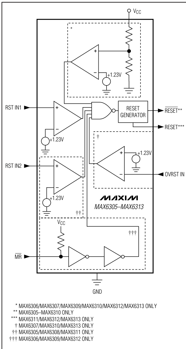
Figure 1. Functional Diagram
