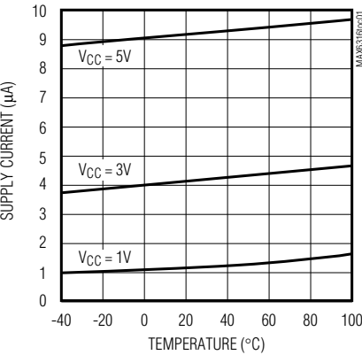
MAX6316/MAX6317/MAX6318/MAX6320/MAX6321 SUPPLY CURRENT vs. TEMPERATURE
