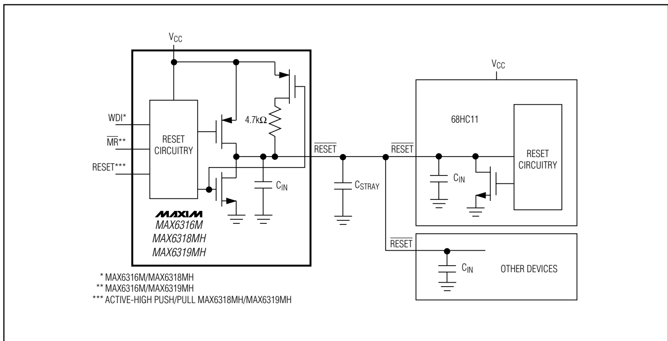
Figure 3. MAX6316M/MAX6318MH/MAX6319MH Supports Additional Devices on the Reset Bus
