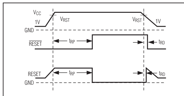
Figure 2. Reset Timing Diagram
