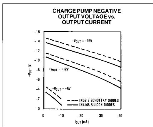
Figure 5. Charge Pump Negative Output Voltage vs. Current
