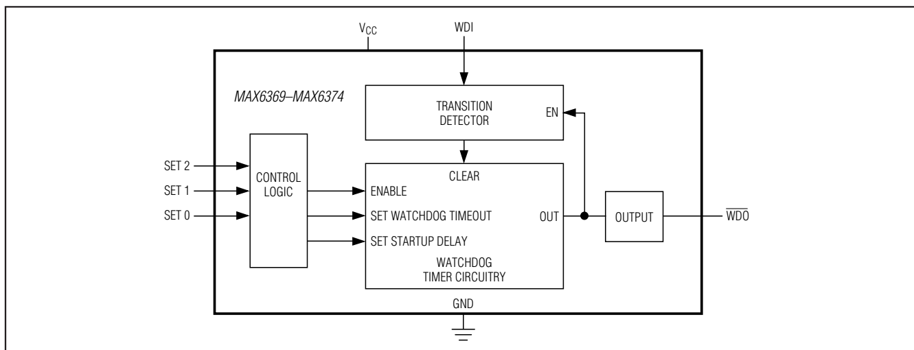
Figure 1. Functional Diagram
