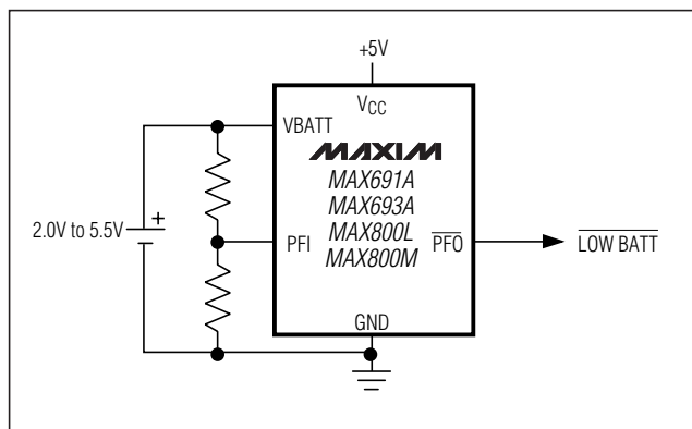
Figure 7. Low-Battery Indicator
